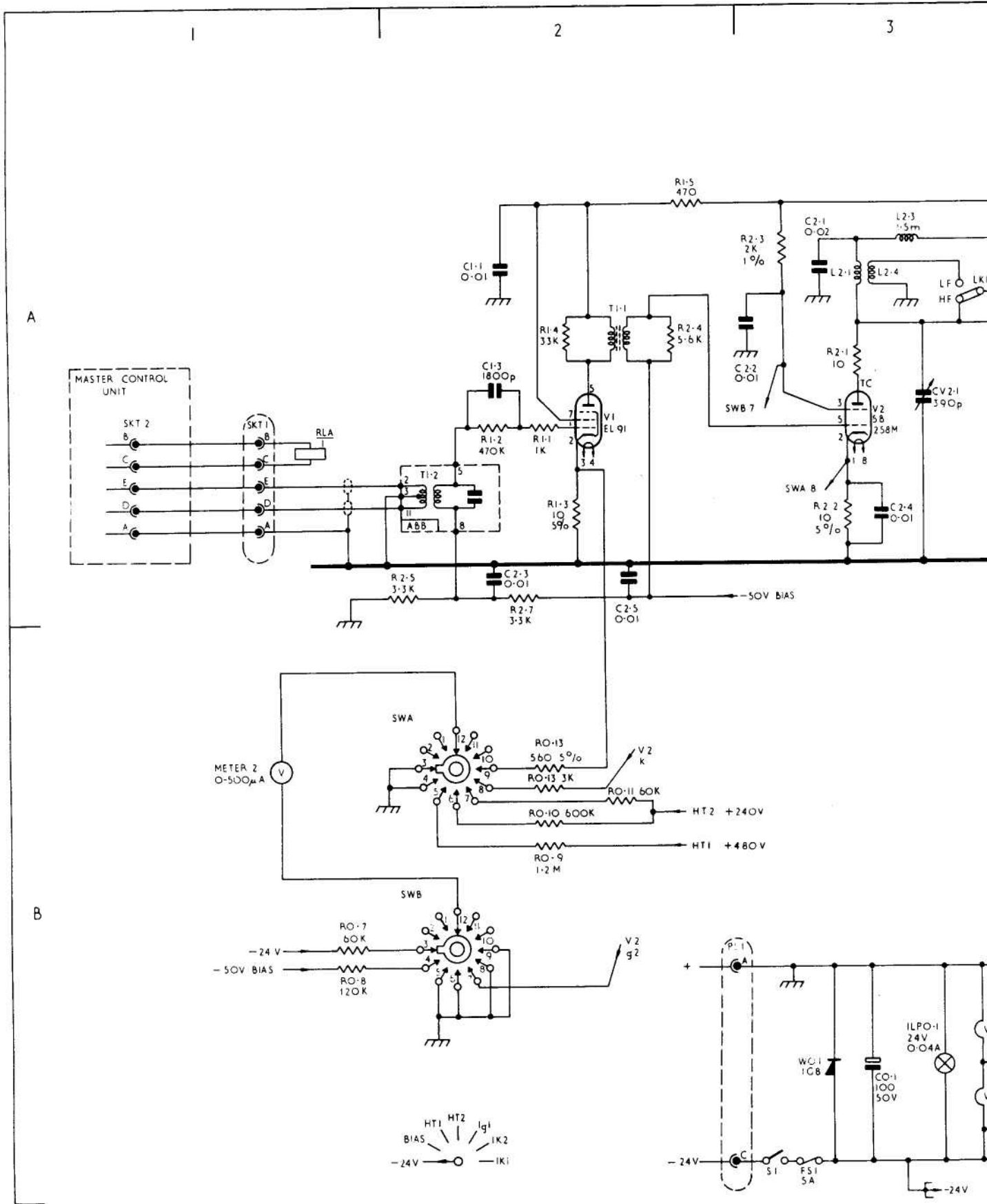
Fig. 9 Transmitter (Type 93)
